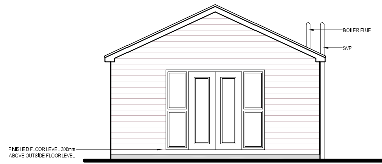
PROPOSED FRONT FACING ELEVATION
